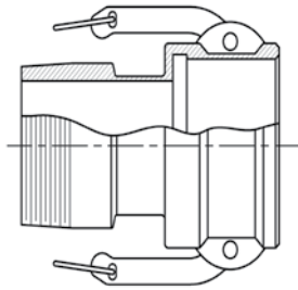
FEMALE CAMLOCK X MALE NPT
