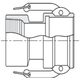
FEMALE CAMLOCK X FEMALE NPT
